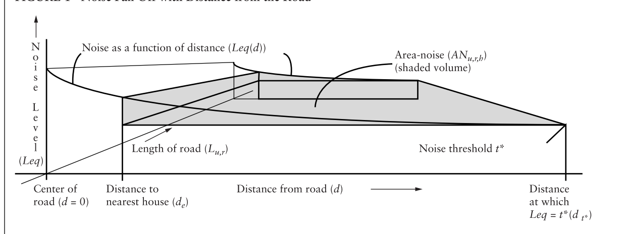
FIGURE 1 Noise Fall Off with Distance from the Road
